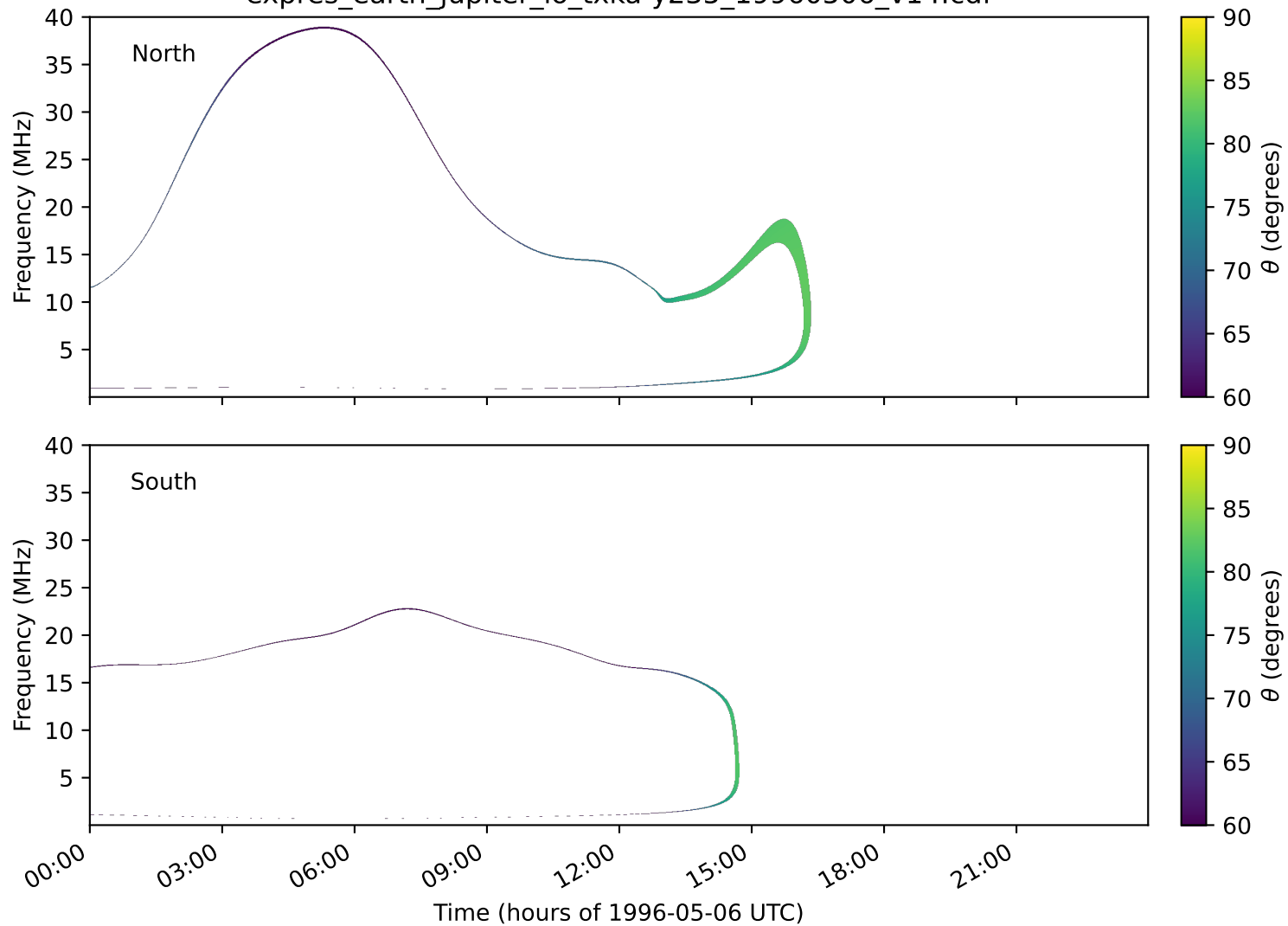
expres_earth_jupiter_io_txka-y235_19960506_v14.cdf
