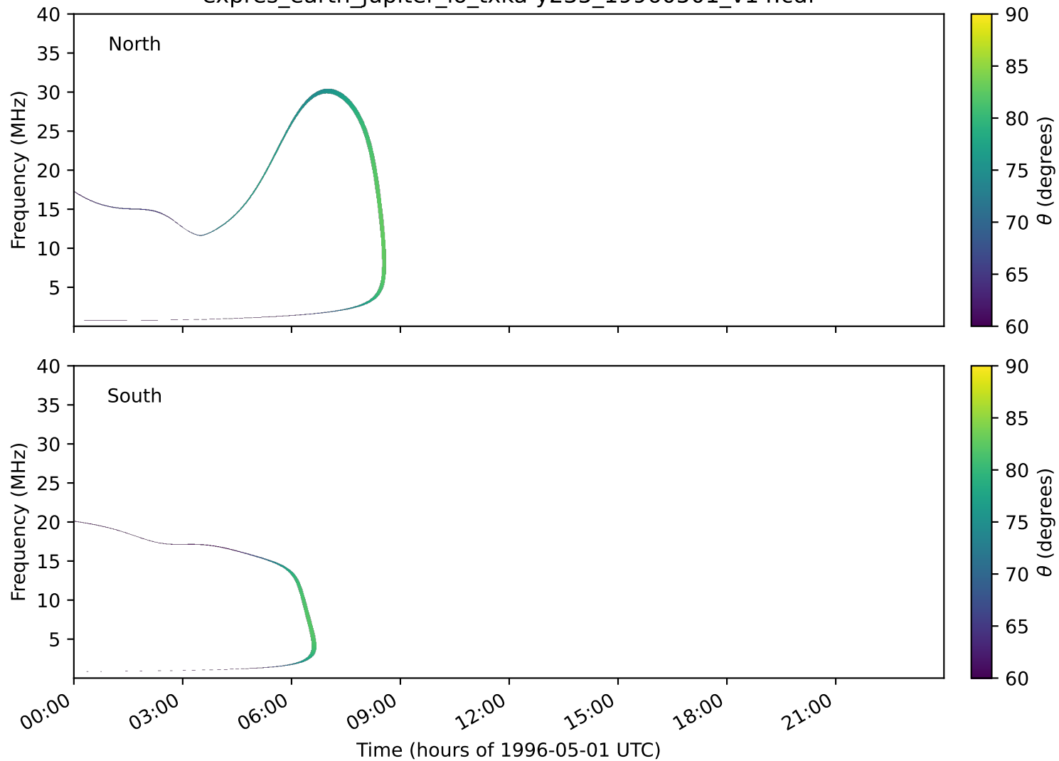
expres_earth_jupiter_io_txka-y235_19960501_v14.cdf
