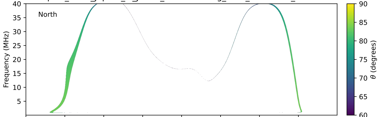
expres_earth_jupiter_io_jrm33_lossc-wid1deg_3kev_19960527_v11.cdf
