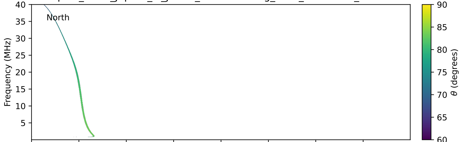
expres_earth_jupiter_io_jrm33_lossc-wid1deg_3kev_19960510_v11.cdf
