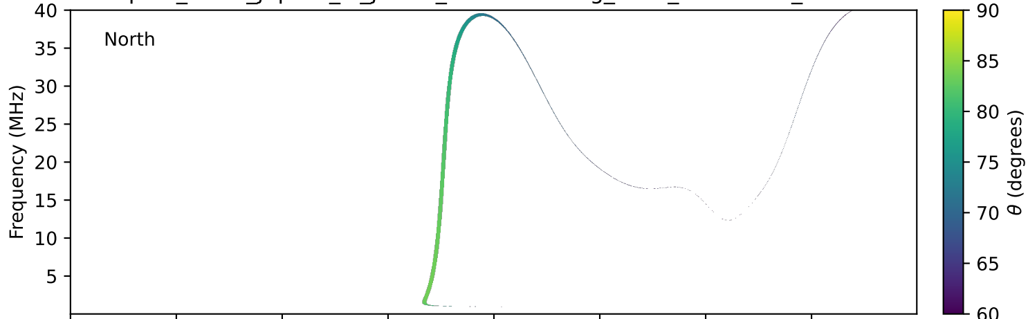
expres_earth_jupiter_io_jrm33_lossc-wid1deg_3kev_19960509_v11.cdf
