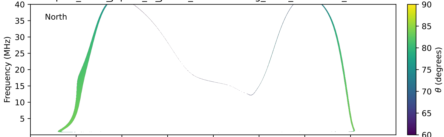
expres_earth_jupiter_io_jrm09_lossc-wid1deg_3kev_19960527_v11.cdf
