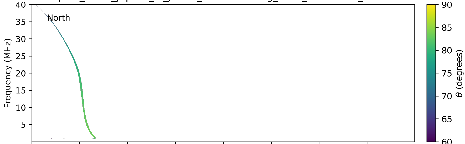
expres_earth_jupiter_io_jrm09_lossc-wid1deg_3kev_19960510_v11.cdf
