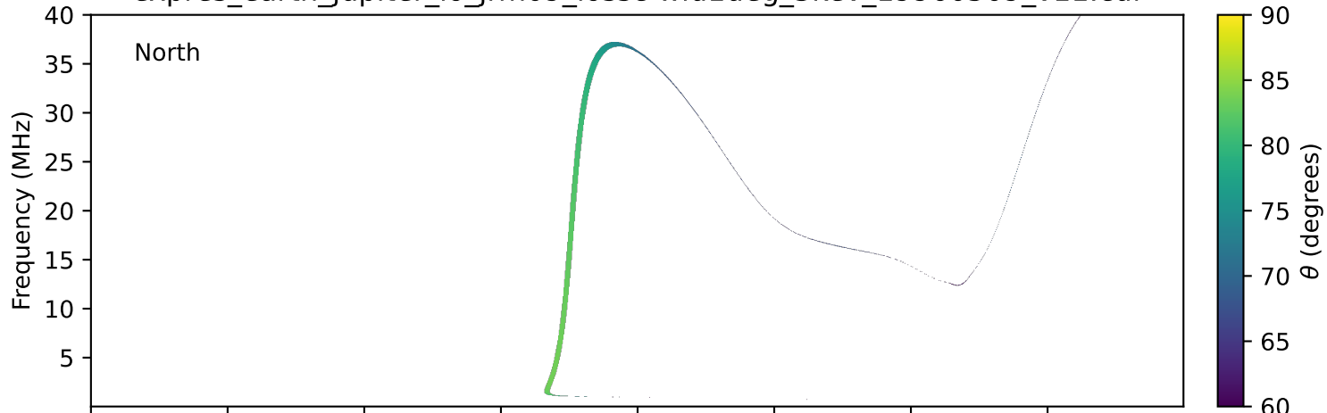
expres_earth_jupiter_io_jrm09_lossc-wid1deg_3kev_19960509_v11.cdf
