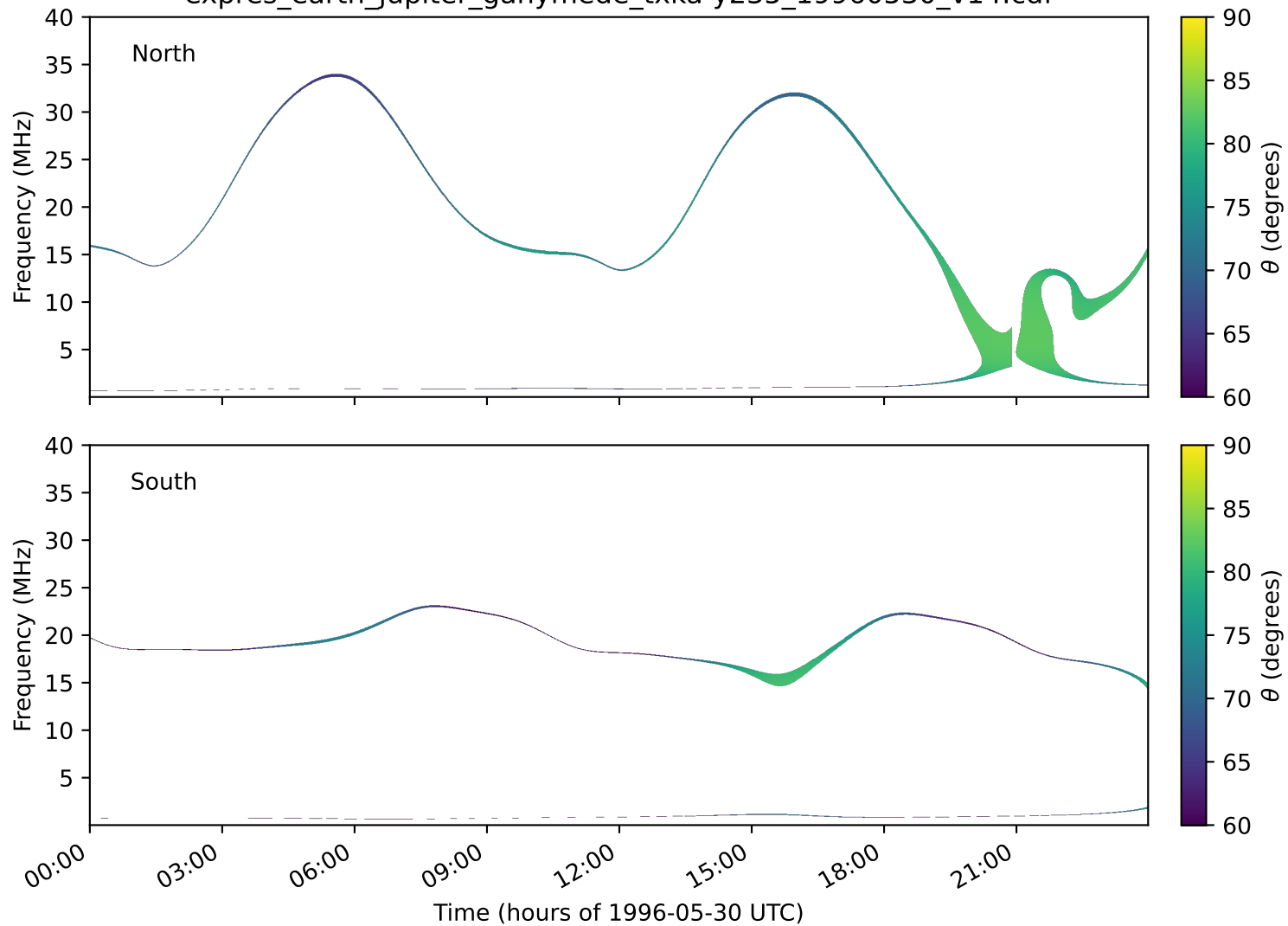
expres_earth_jupiter_ganymede_txka-y235_19960530_v14.cdf
