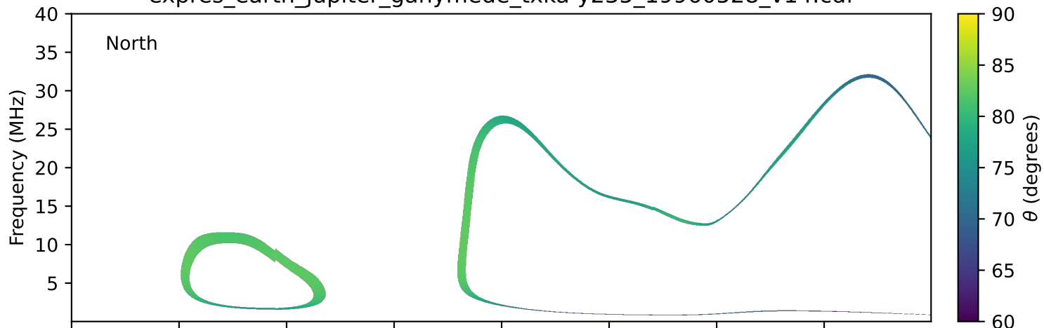
expres_earth_jupiter_ganymede_txka-y235_19960528_v14.cdf
