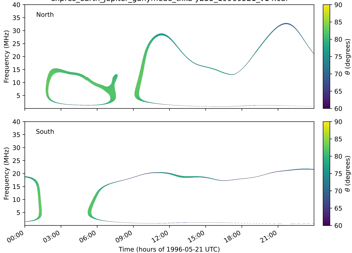
expres_earth_jupiter_ganymede_txka-y235_19960521_v14.cdf
