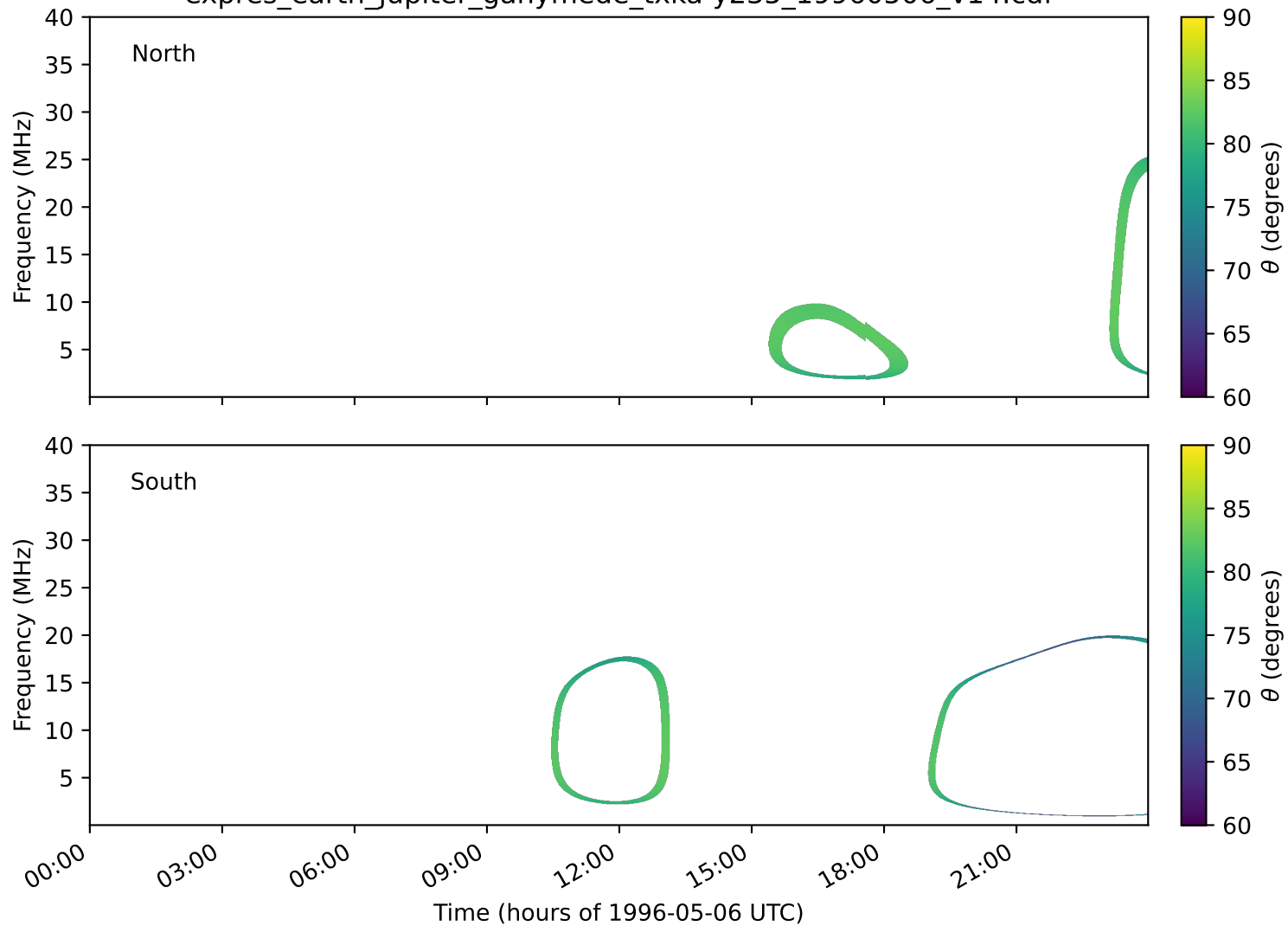
expres_earth_jupiter_ganymede_txka-y235_19960506_v14.cdf
