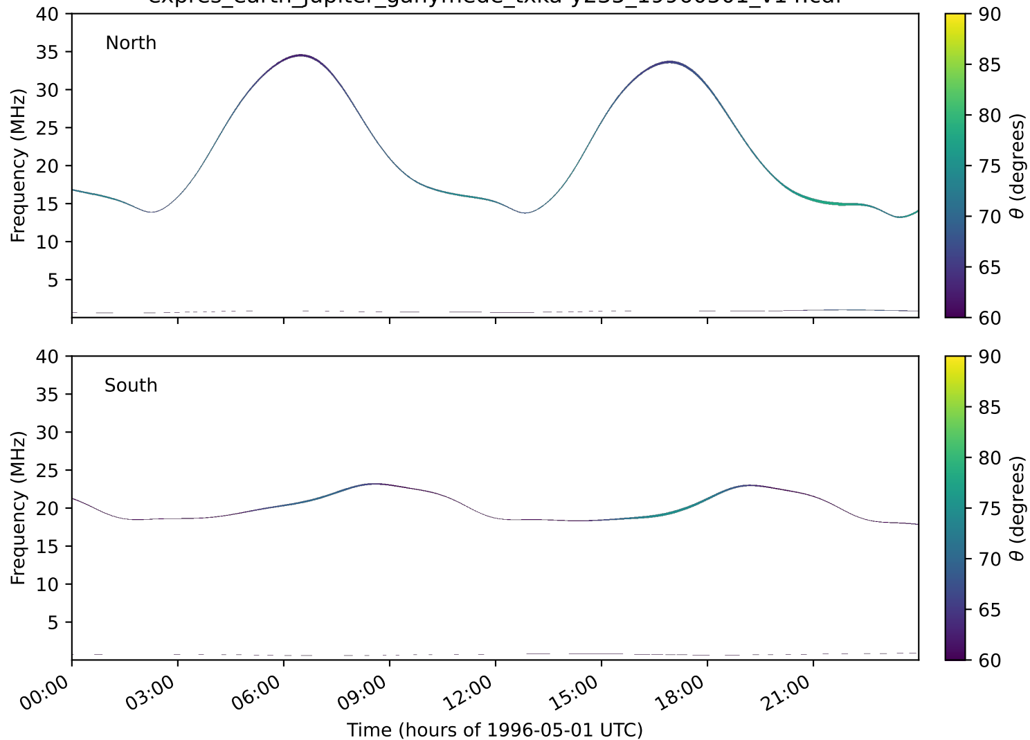
expres_earth_jupiter_ganymede_txka-y235_19960501_v14.cdf
