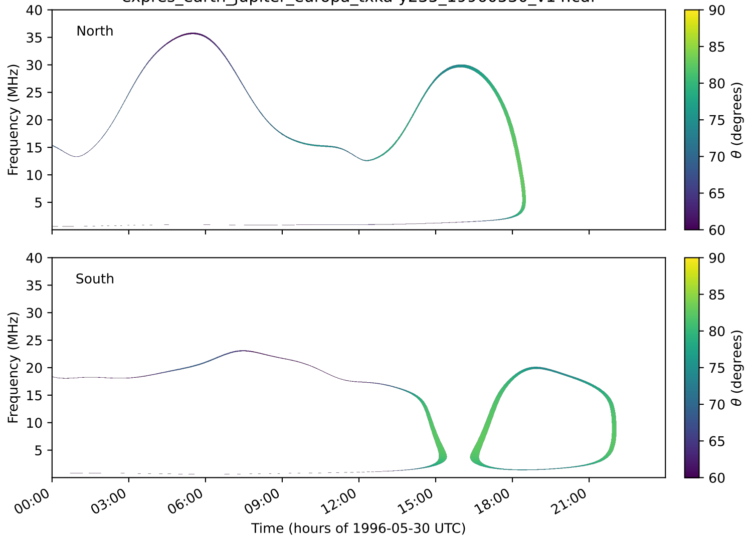
expres_earth_jupiter_europa_txka-y235_19960530_v14.cdf
