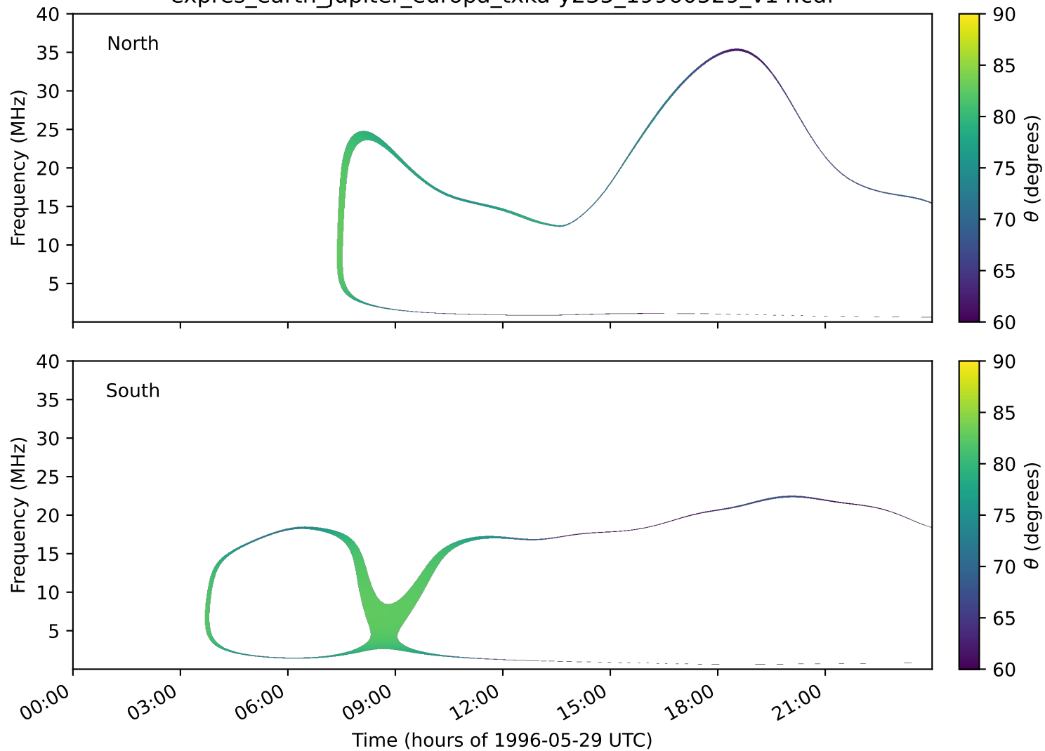
expres_earth_jupiter_europa_txka-y235_19960529_v14.cdf
