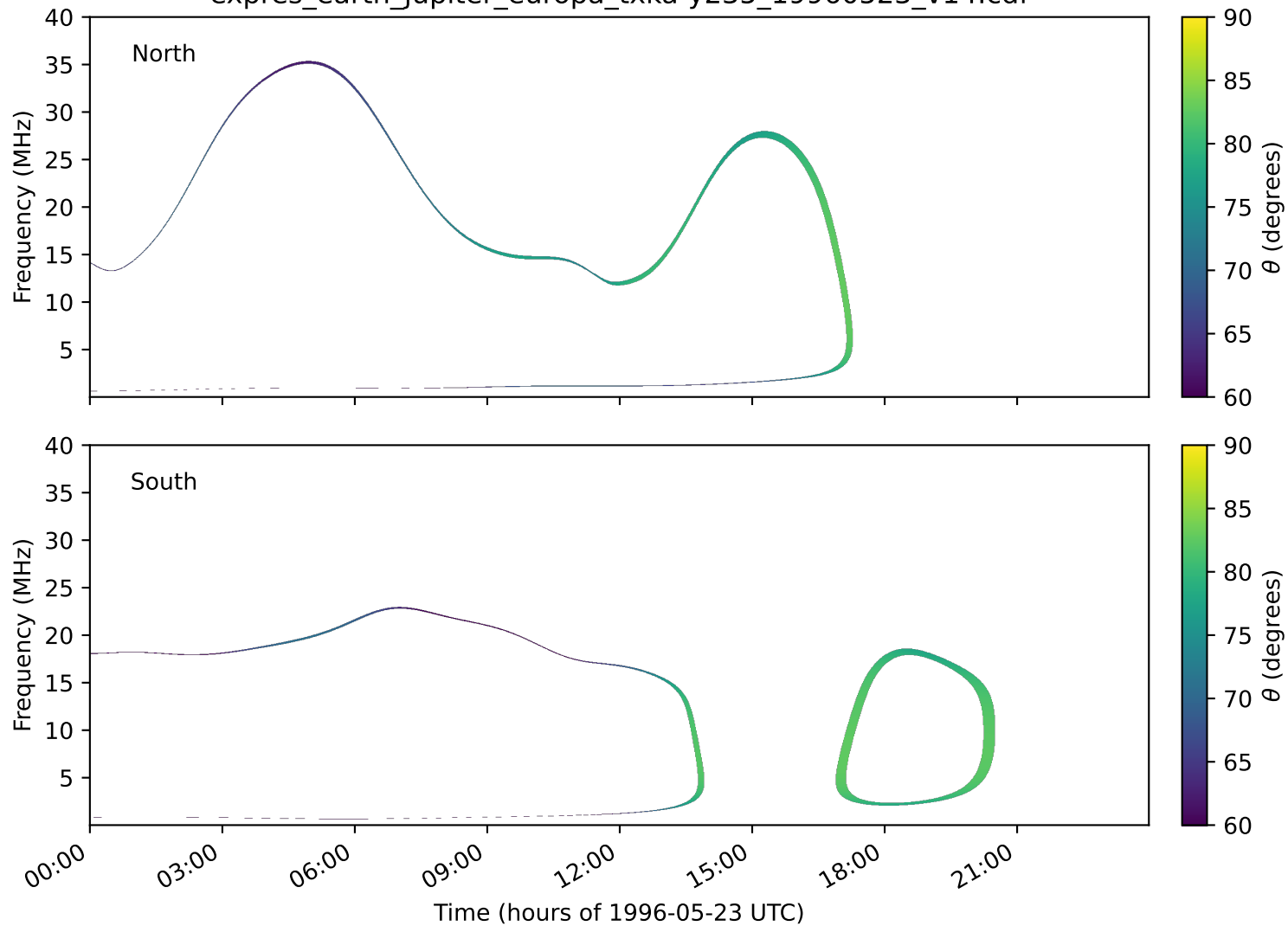
expres_earth_jupiter_europa_txka-y235_19960523_v14.cdf
