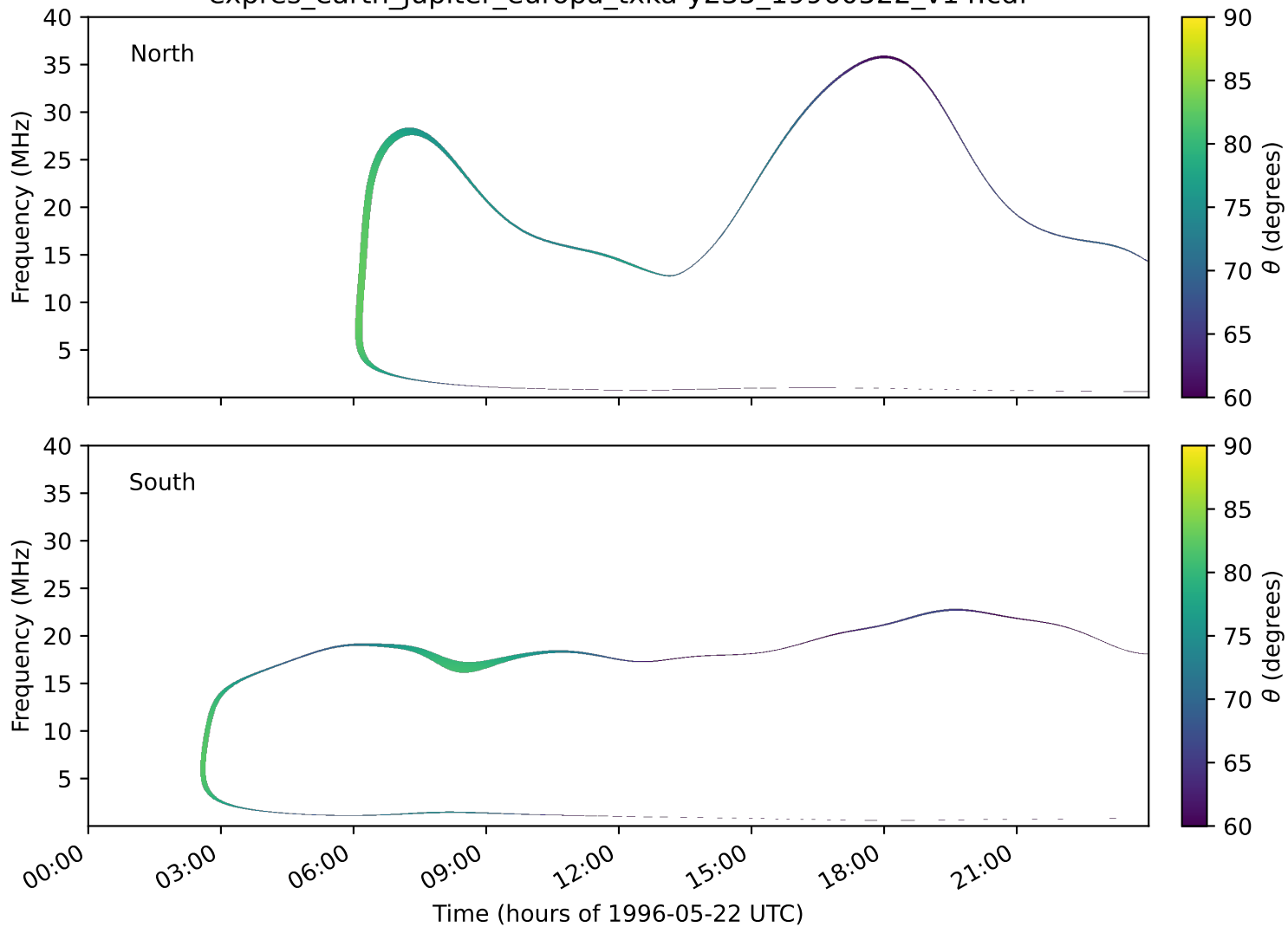
expres_earth_jupiter_europa_txka-y235_19960522_v14.cdf
