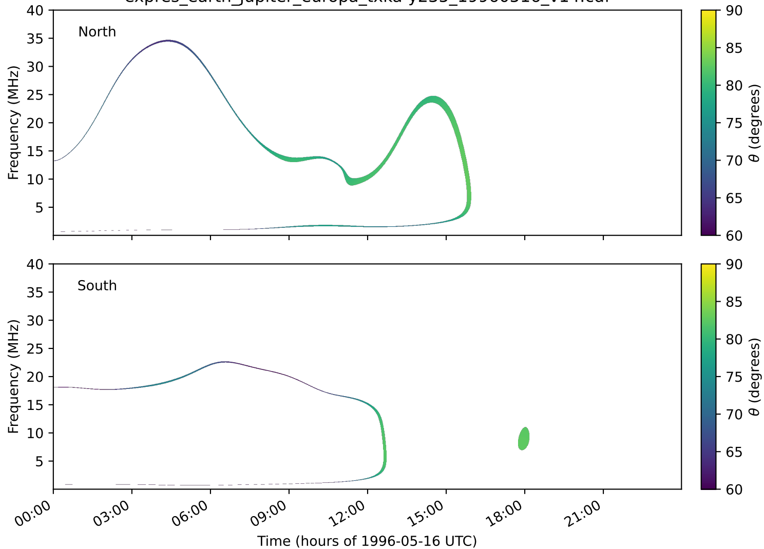
expres_earth_jupiter_europa_txka-y235_19960516_v14.cdf
