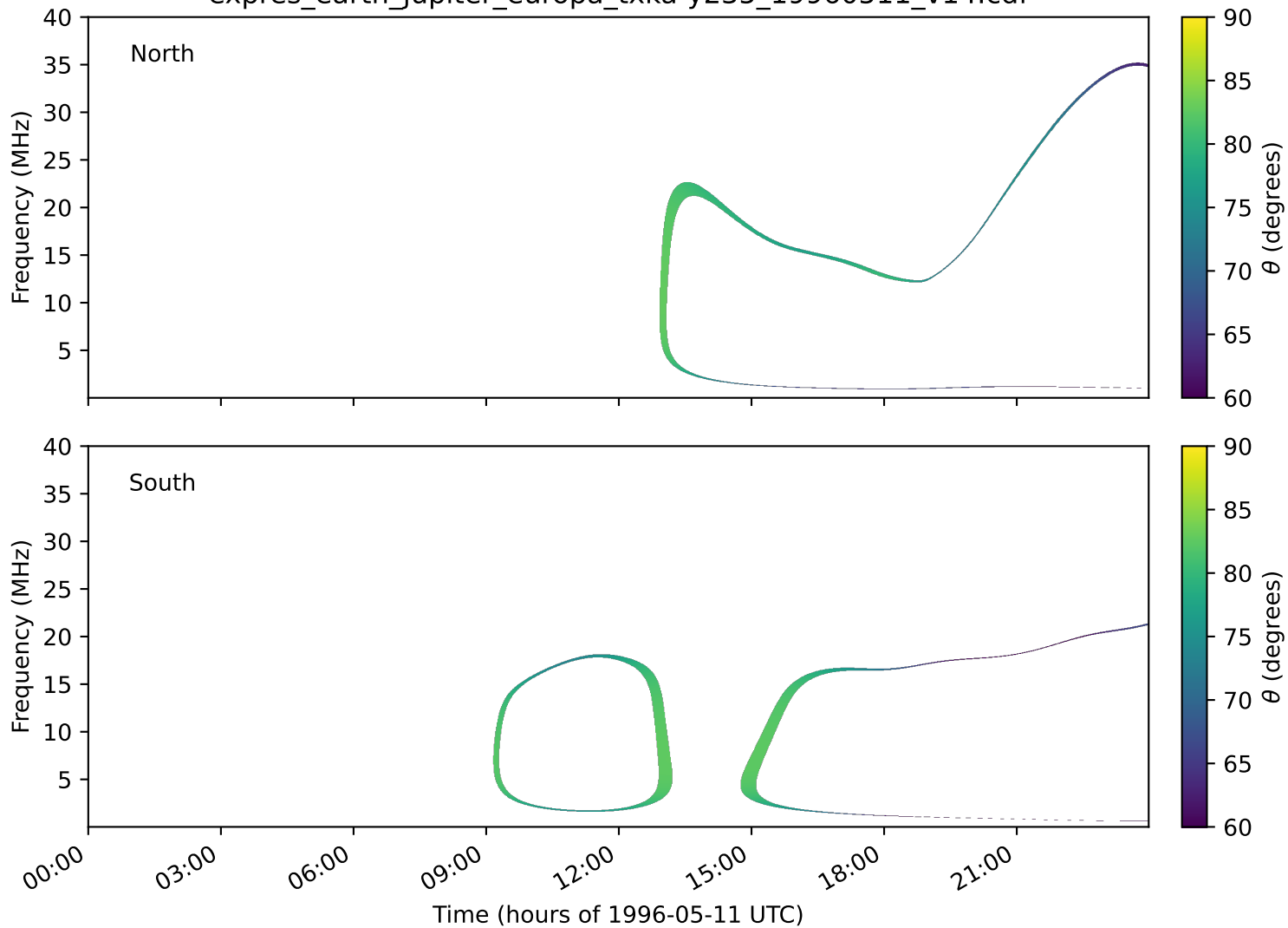
expres_earth_jupiter_europa_txka-y235_19960511_v14.cdf
