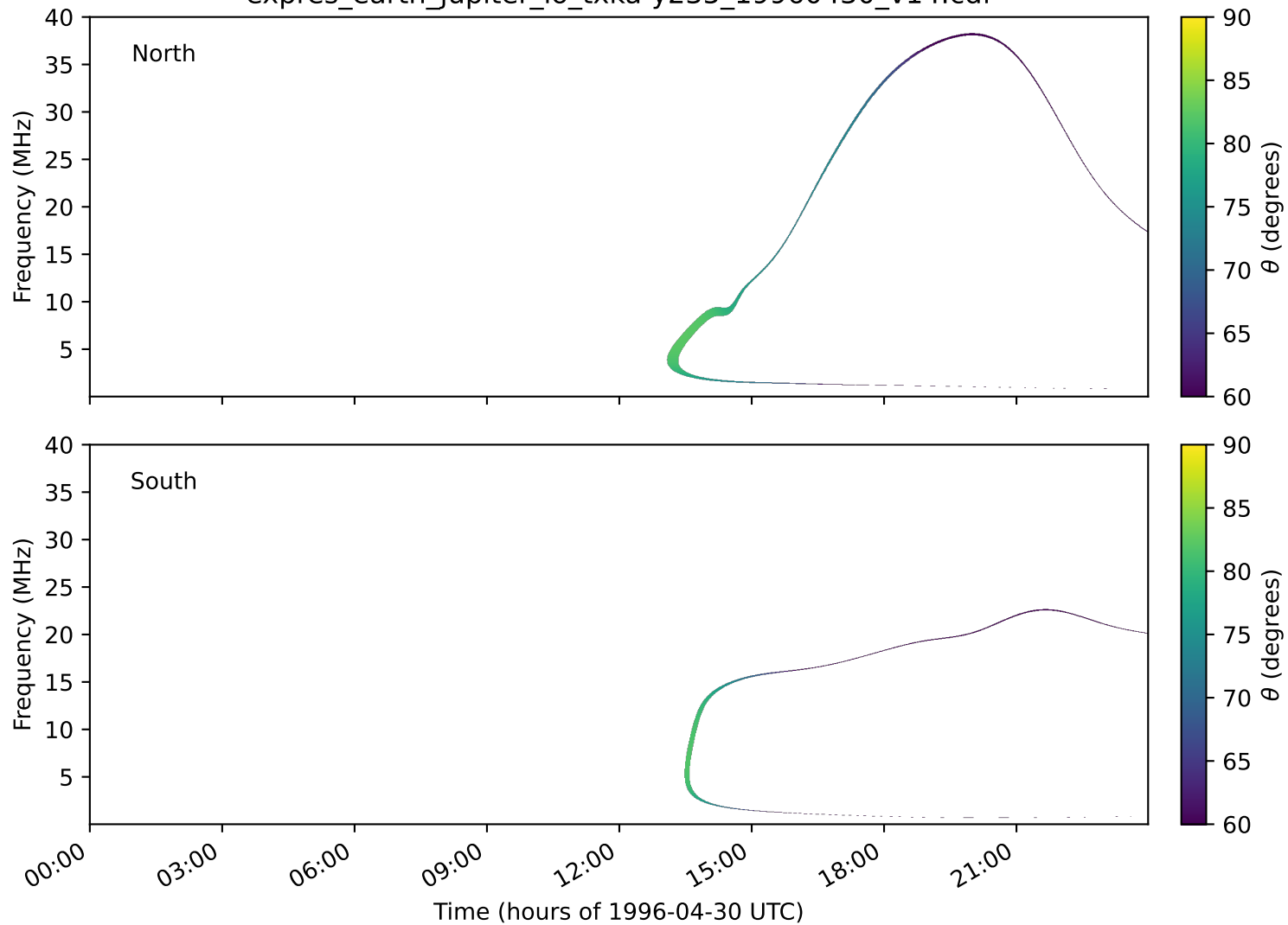
expres_earth_jupiter_io_txka-y235_19960430_v14.cdf
