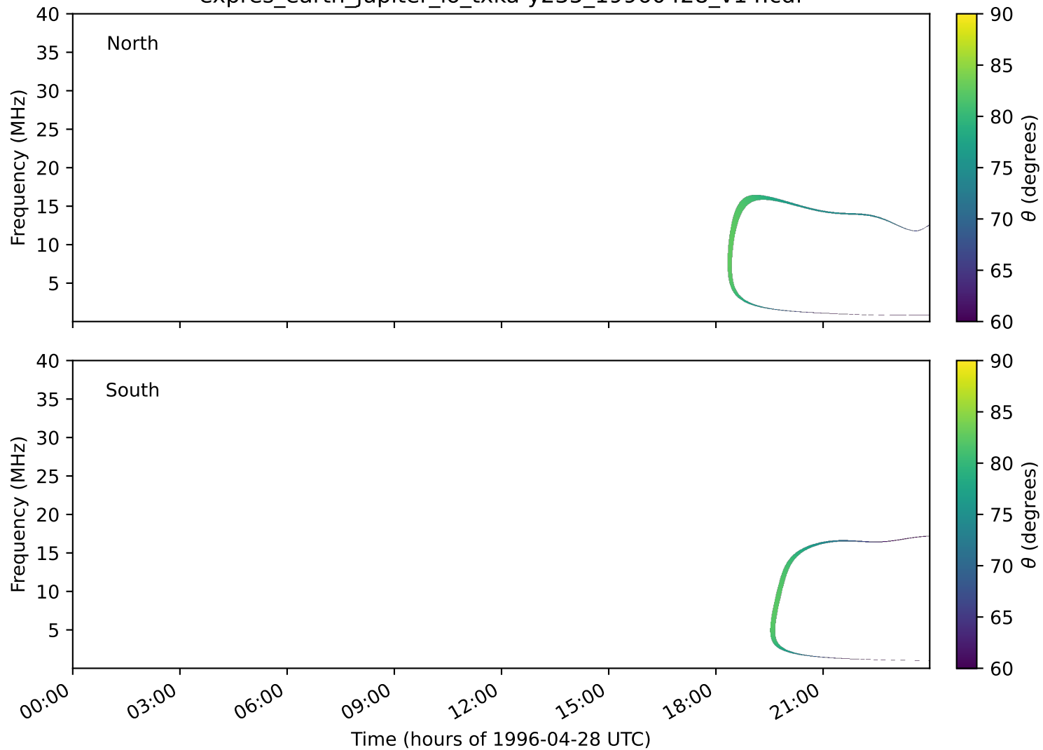
expres_earth_jupiter_io_txka-y235_19960428_v14.cdf
