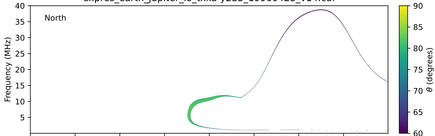
expres_earth_jupiter_io_txka-y235_19960423_v14.cdf
