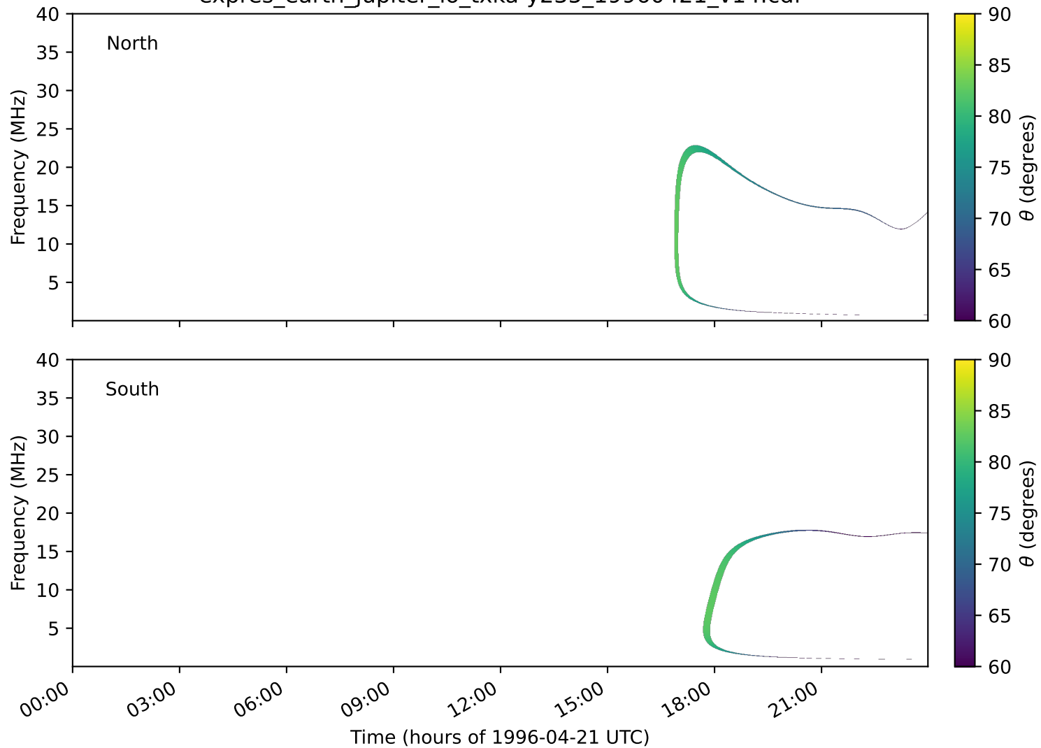
expres_earth_jupiter_io_txka-y235_19960421_v14.cdf
