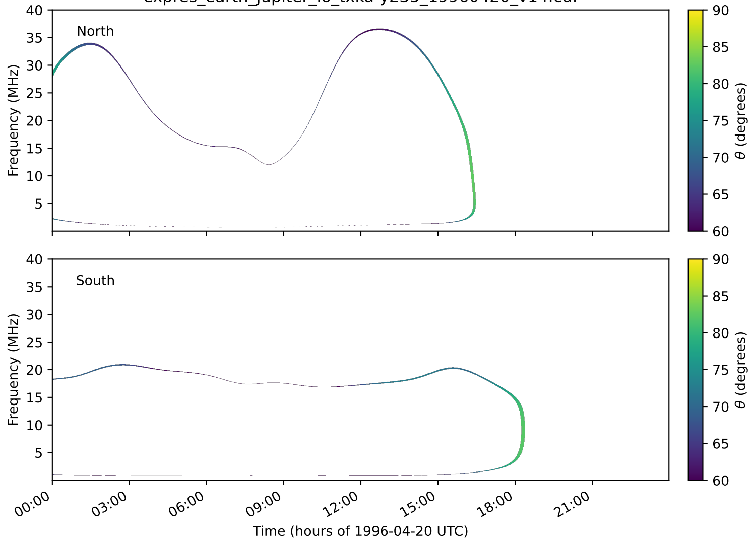
expres_earth_jupiter_io_txka-y235_19960420_v14.cdf
