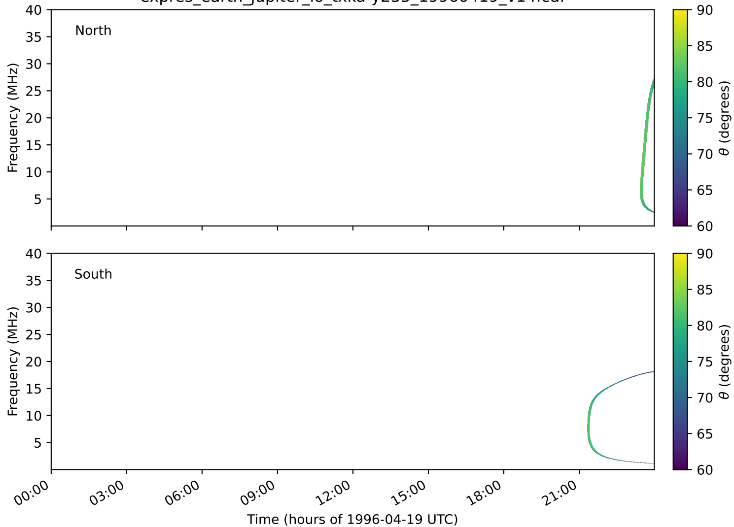
expres_earth_jupiter_io_txka-y235_19960419_v14.cdf
