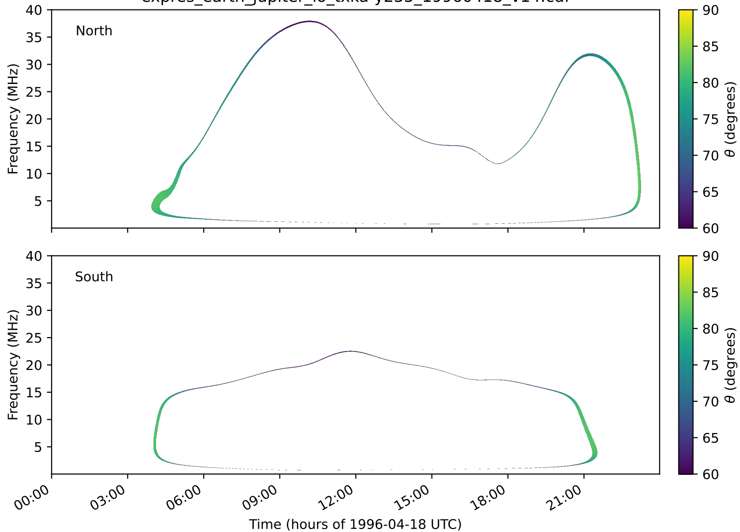
expres_earth_jupiter_io_txka-y235_19960418_v14.cdf
