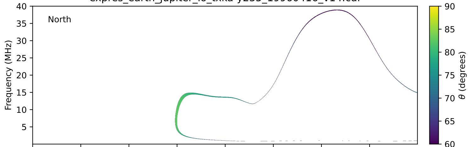
expres_earth_jupiter_io_txka-y235_19960416_v14.cdf
