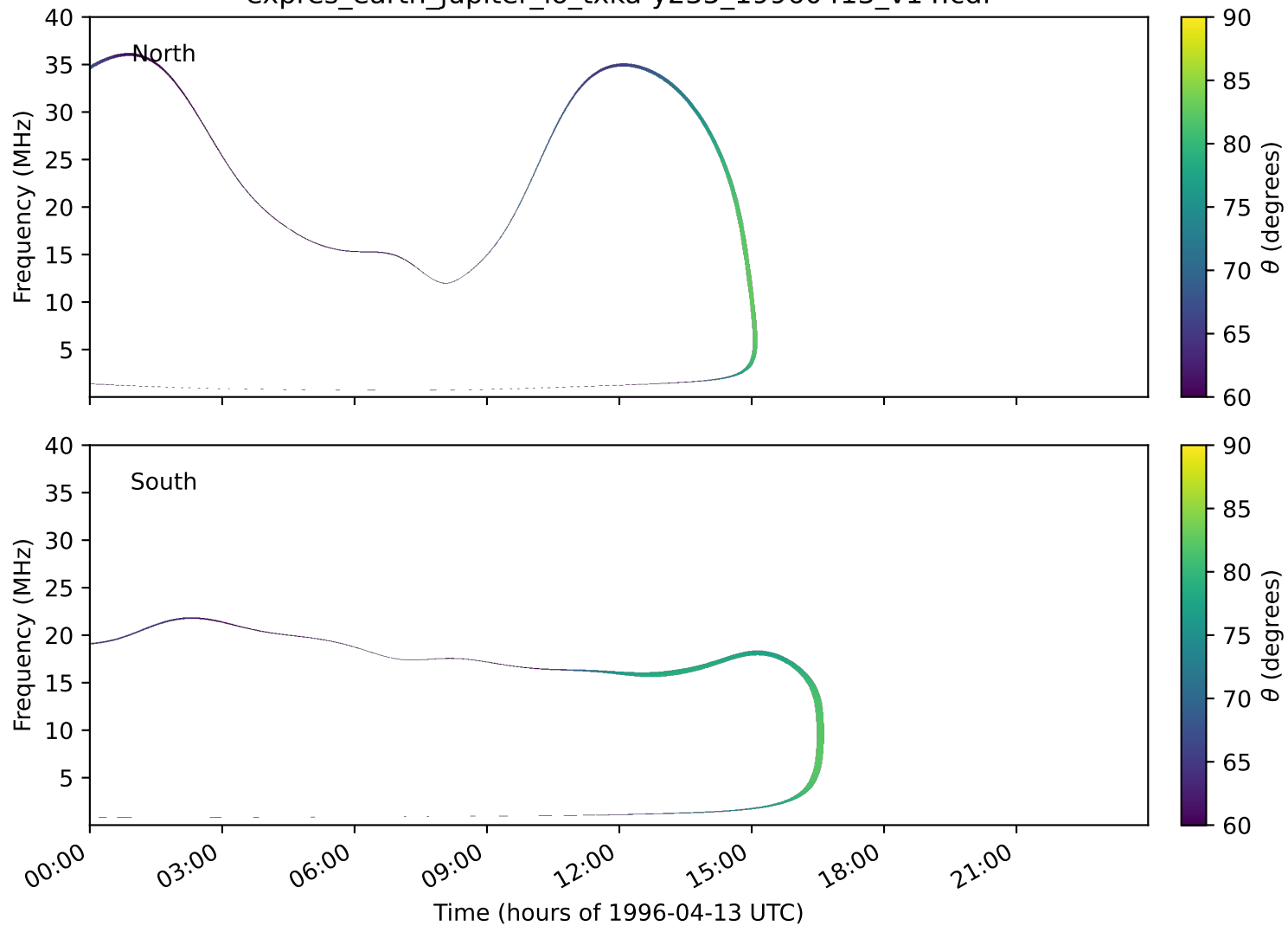
expres_earth_jupiter_io_txka-y235_19960413_v14.cdf
