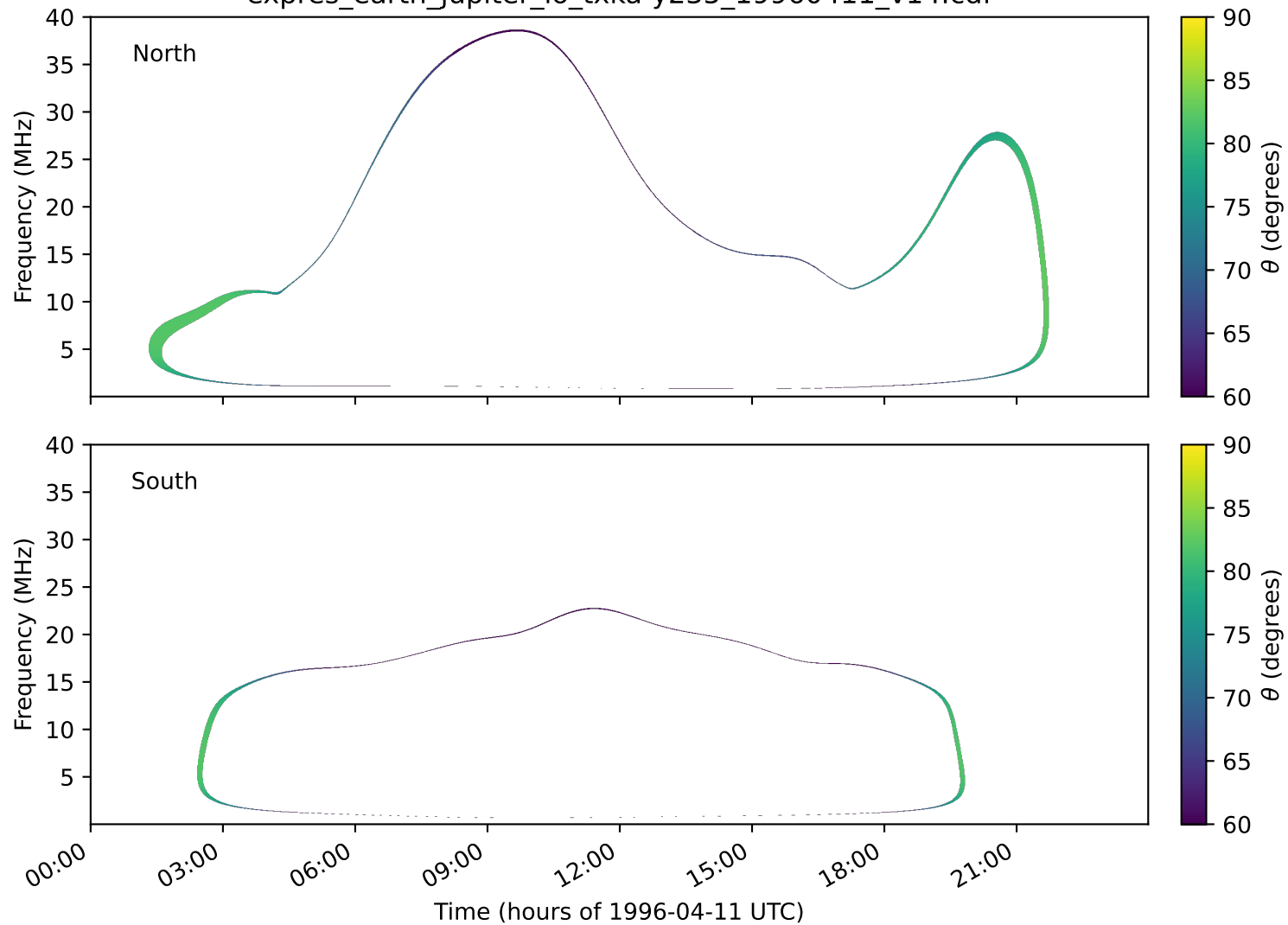
expres_earth_jupiter_io_txka-y235_19960411_v14.cdf
