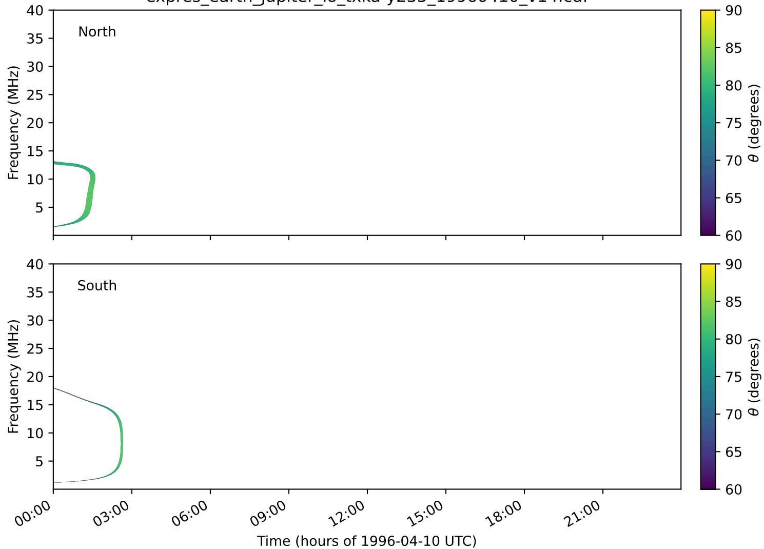
expres_earth_jupiter_io_txka-y235_19960410_v14.cdf
