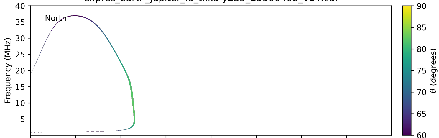
expres_earth_jupiter_io_txka-y235_19960408_v14.cdf
