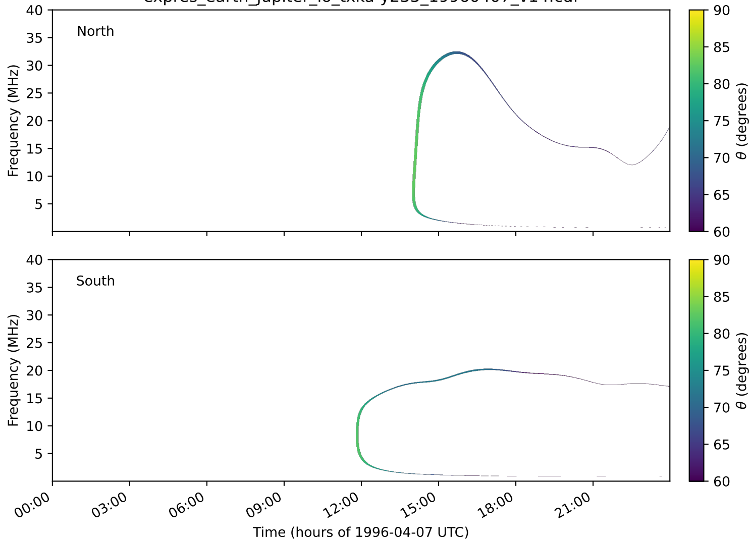
expres_earth_jupiter_io_txka-y235_19960407_v14.cdf
