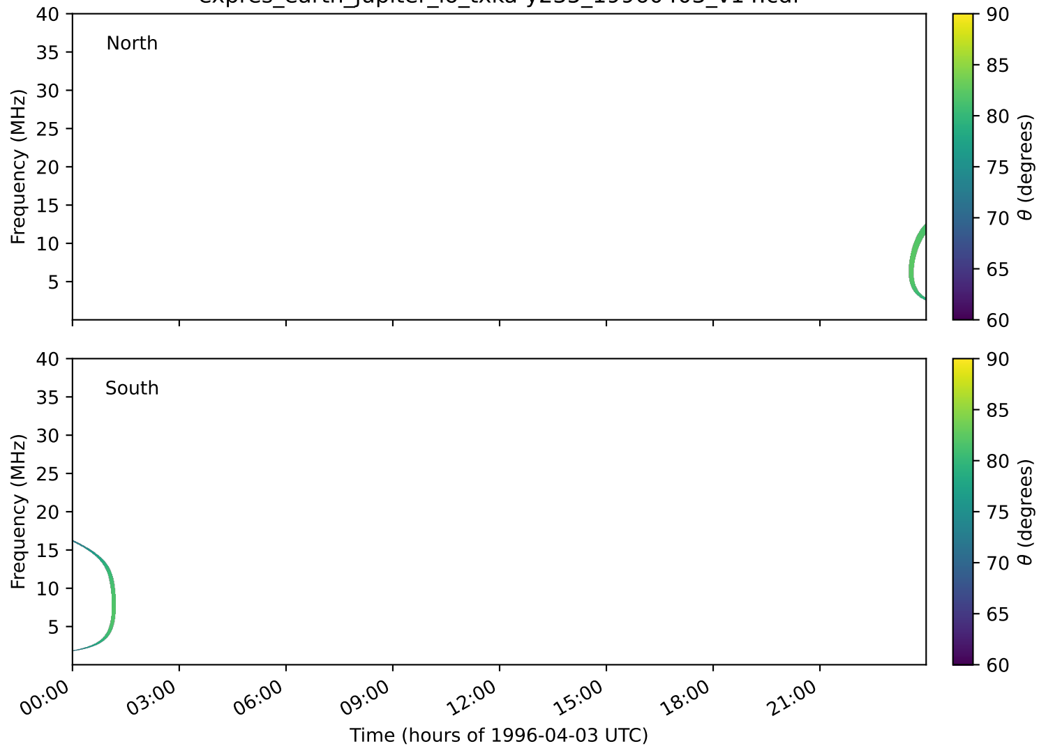
expres_earth_jupiter_io_txka-y235_19960403_v14.cdf
