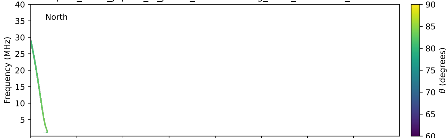
expres_earth_jupiter_io_jrm33_lossc-wid1deg_3kev_19960426_v11.cdf
