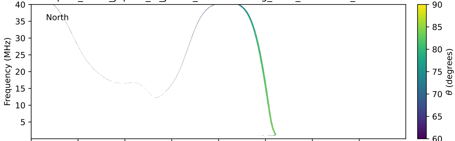
expres_earth_jupiter_io_jrm33_lossc-wid1deg_3kev_19960413_v11.cdf
