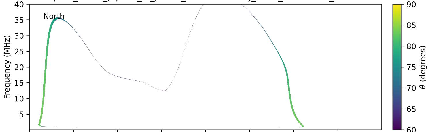
expres_earth_jupiter_io_jrm09_lossc-wid1deg_3kev_19960427_v11.cdf
