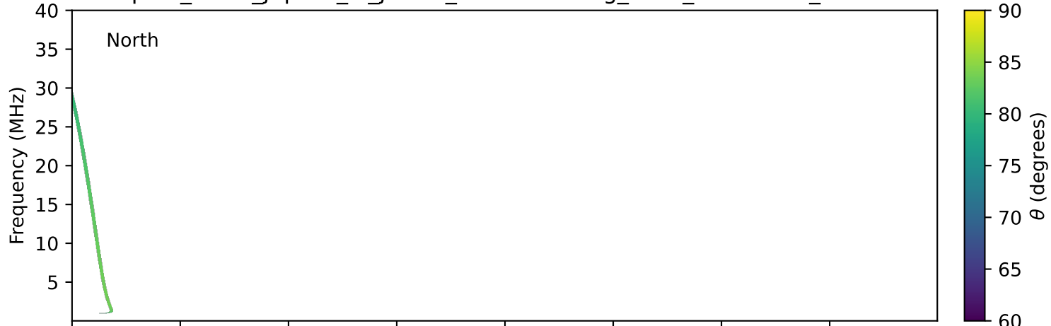
expres_earth_jupiter_io_jrm09_lossc-wid1deg_3kev_19960426_v11.cdf
