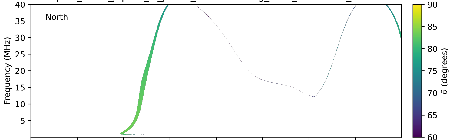
expres_earth_jupiter_io_jrm09_lossc-wid1deg_3kev_19960425_v11.cdf
