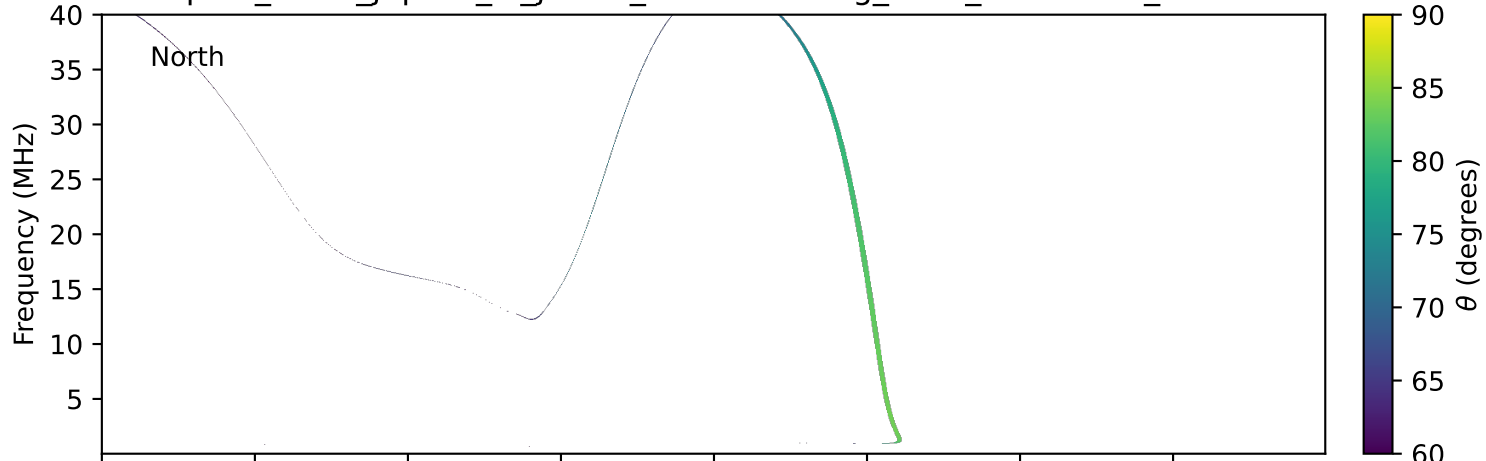
expres_earth_jupiter_io_jrm09_lossc-wid1deg_3kev_19960413_v11.cdf
