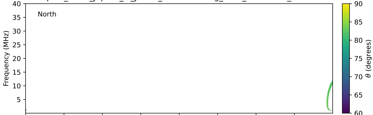
expres_earth_jupiter_io_jrm09_lossc-wid1deg_3kev_19960403_v11.cdf
