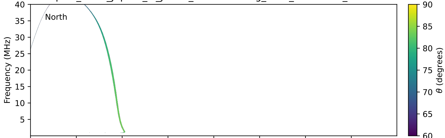
expres_earth_jupiter_io_jrm09_lossc-wid1deg_3kev_19960401_v11.cdf
