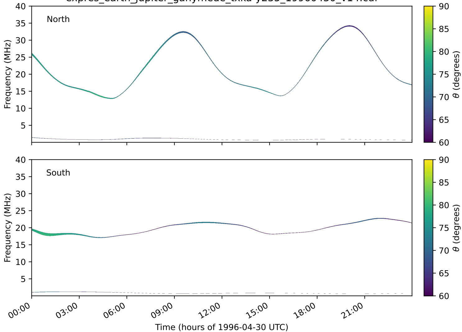
expres_earth_jupiter_ganymede_txka-y235_19960430_v14.cdf
