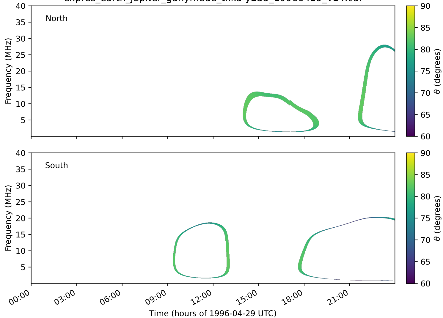
expres_earth_jupiter_ganymede_txka-y235_19960429_v14.cdf
