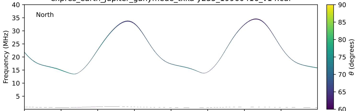
expres_earth_jupiter_ganymede_txka-y235_19960416_v14.cdf
