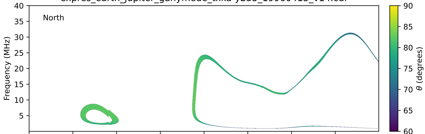
expres_earth_jupiter_ganymede_txka-y235_19960415_v14.cdf
