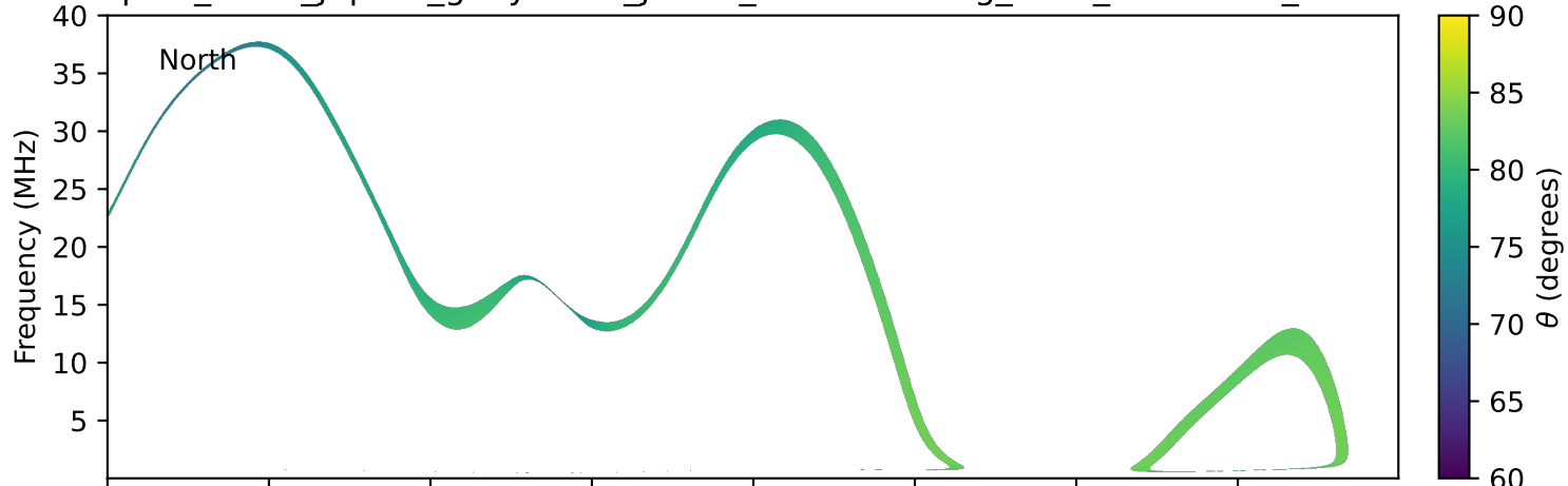
expres_earth_jupiter_ganymede_jrm33_lossc-wid1deg_3kev_19960425_v11.cdf
