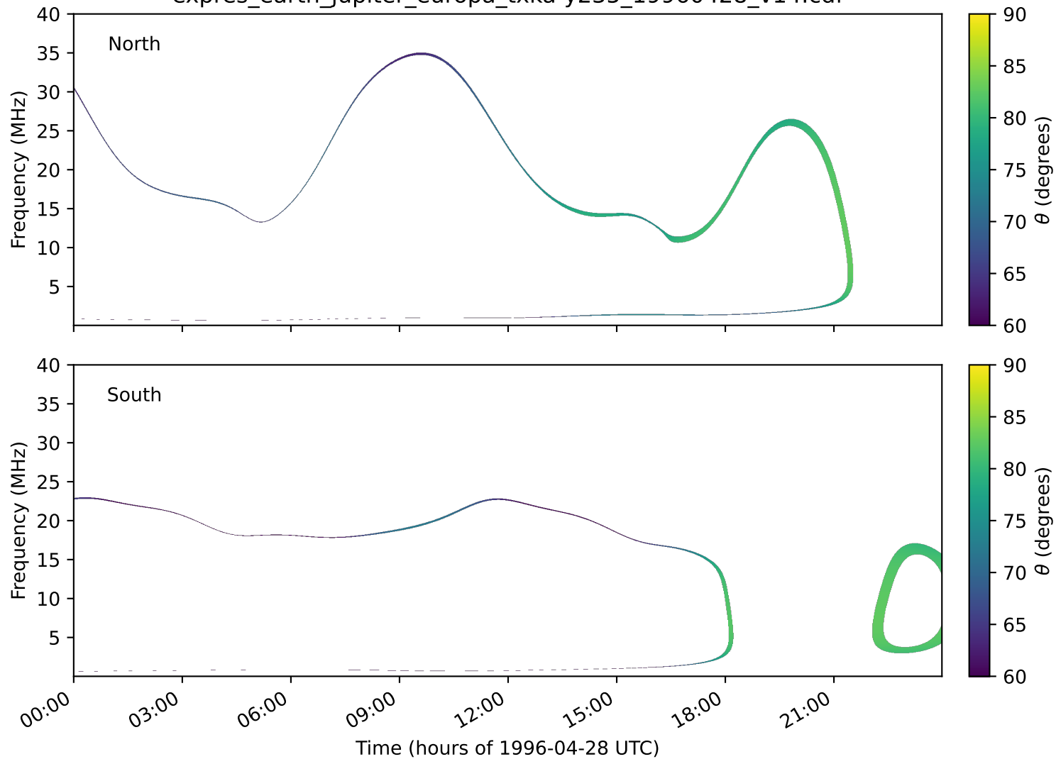
expres_earth_jupiter_europa_txka-y235_19960428_v14.cdf
