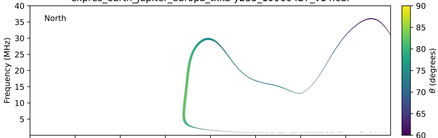
expres_earth_jupiter_europa_txka-y235_19960427_v14.cdf
