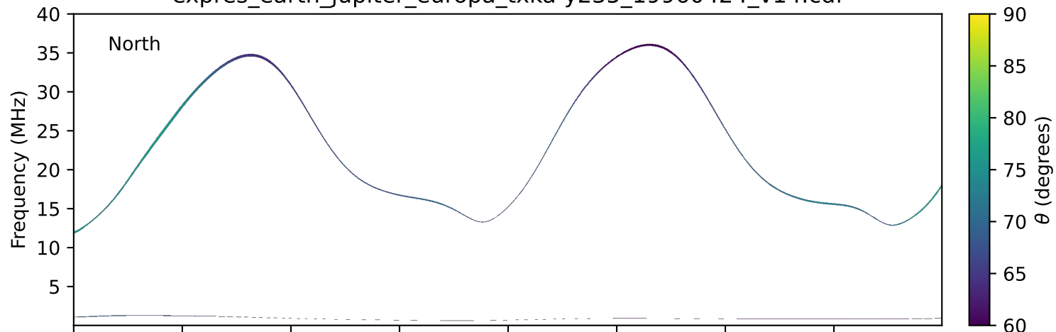
expres_earth_jupiter_europa_txka-y235_19960424_v14.cdf
