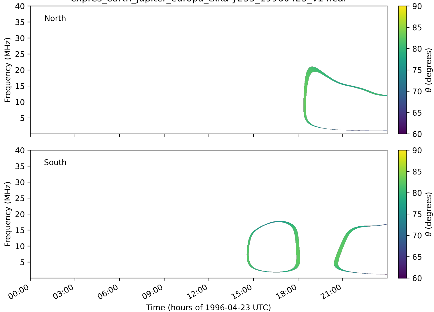
expres_earth_jupiter_europa_txka-y235_19960423_v14.cdf
